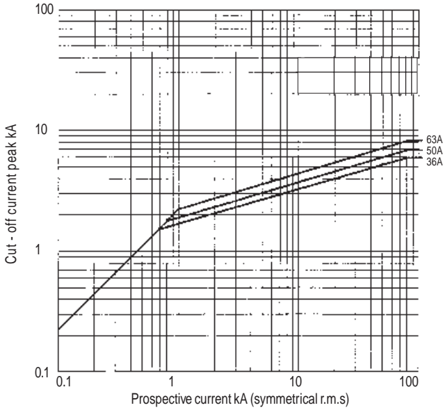
Cut-off characteristics
