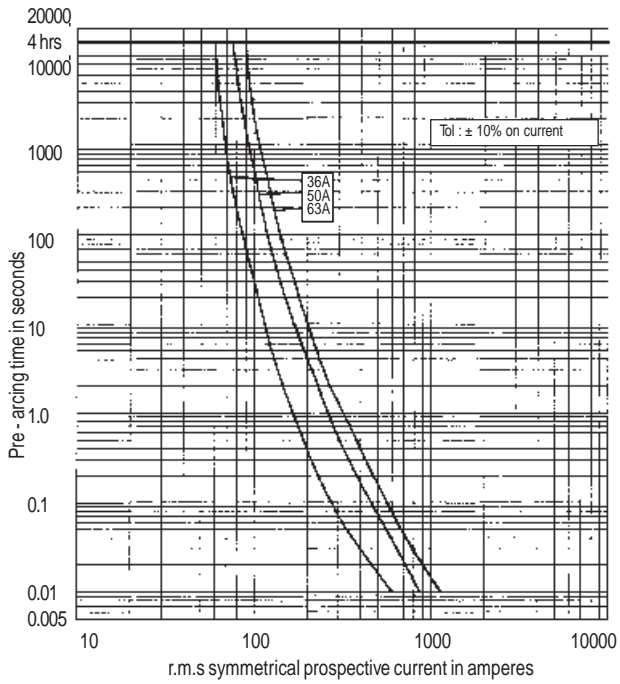
Time current characteristics
